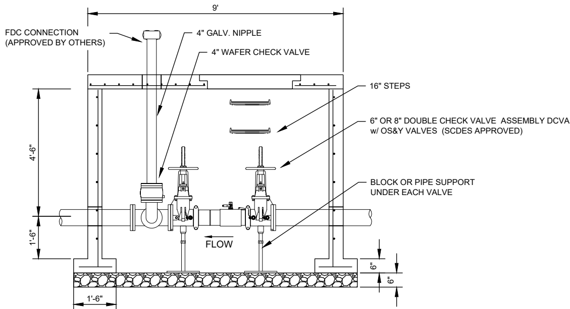
ELEVATION VIEW
