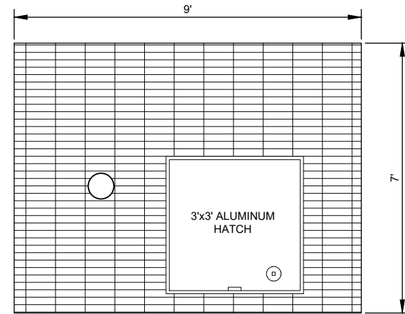
TOP SLAB
